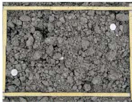
Abb. 10: ideales Saatbeet.
